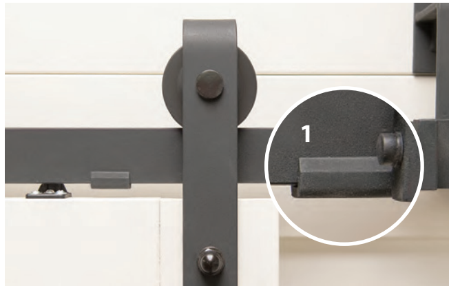
1. Easy Clip Soft Close attachment discretely hidden behind track
